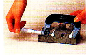
Measuring dovetail
